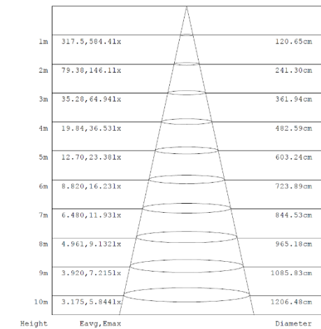
Diaqram for RULFA-01 in 6W, 4000K Other diaqramms available on request
